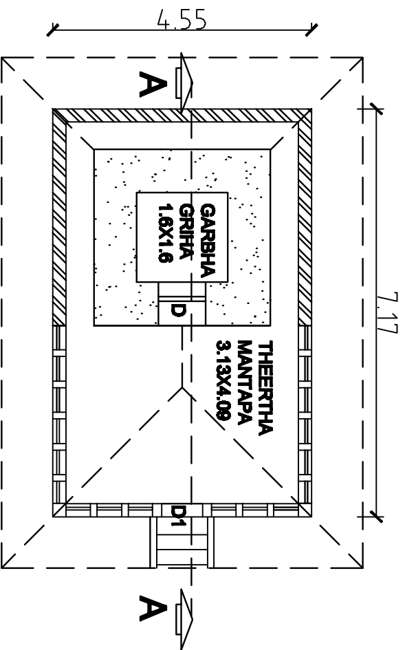
FLOOR PLAN SCALE 1:100
